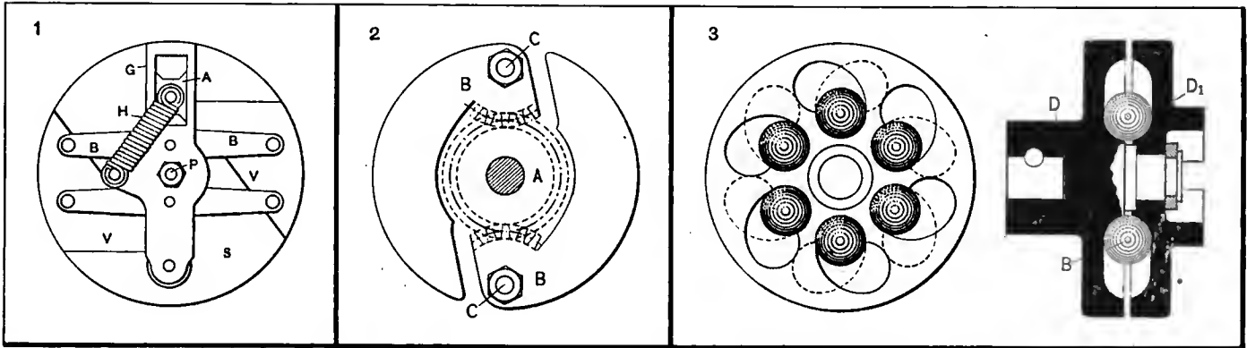
Fig. 1.—Timing the break of primary current Fig. 2.—Turning armature by swinging weights Fig. 3.—Curved sockets in multiple ball coupling of the Ruthardt Magneto
